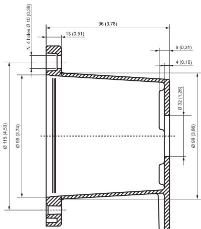
Pump side
