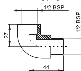
90° adapter for vertical tanks filling plug
