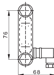
Electric thermostatic level gauge
