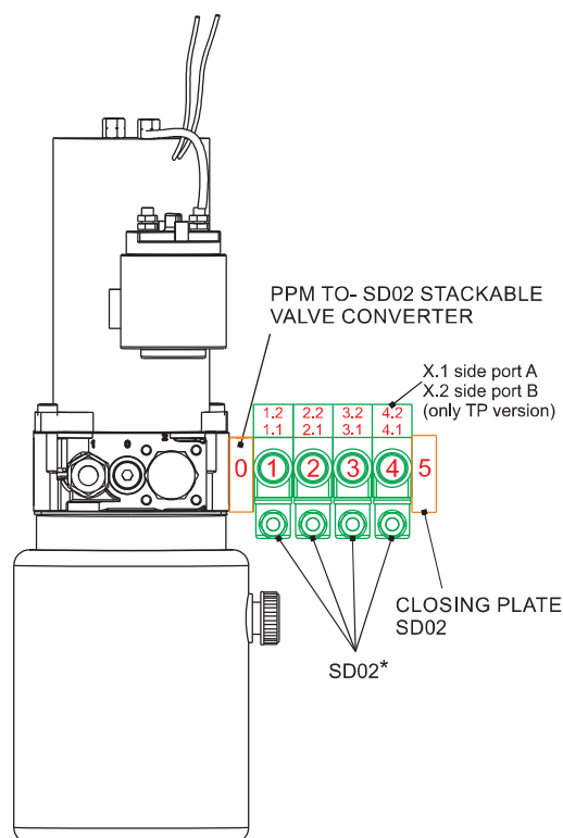
PPM + SD02 STACKABLE VALVES
