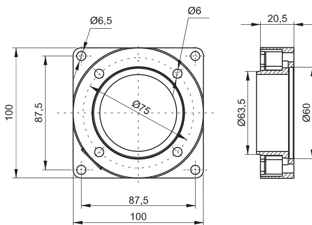
Adaptor flange
