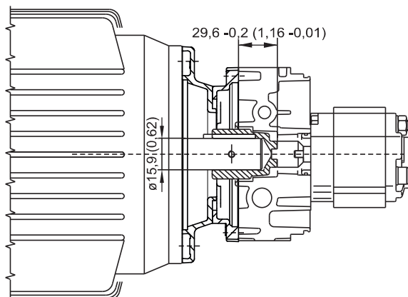
Couplings
