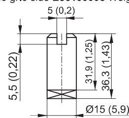
Couplings
