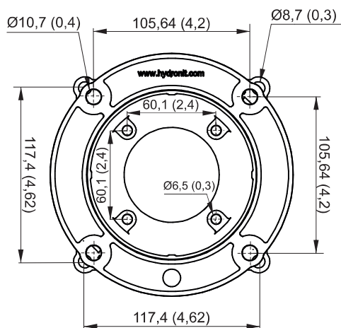
Adaptor flange
