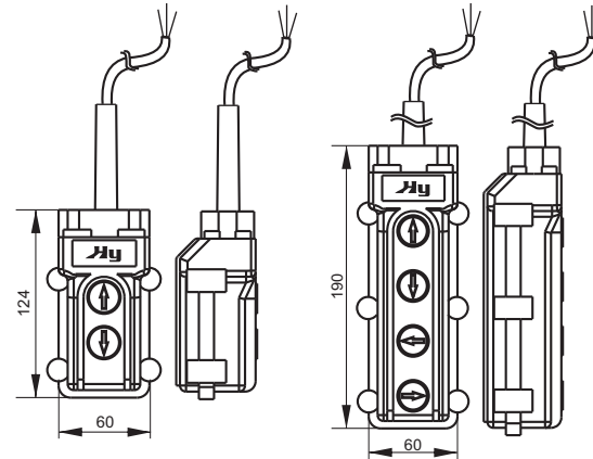
Wired remote control Weight: 0,60 kg Max Current @ Voltage: Protection degree: IP65 2A@400VAC; 5A@220VAC/24VDC/12VDC
