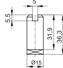
Motor side E36100002 Weight: 0,12 Kg
