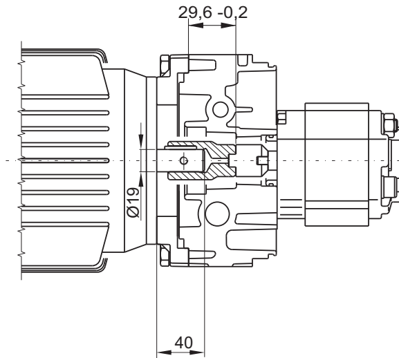
Pump side (group1) E36100000 Weight: 0,05 Kg
