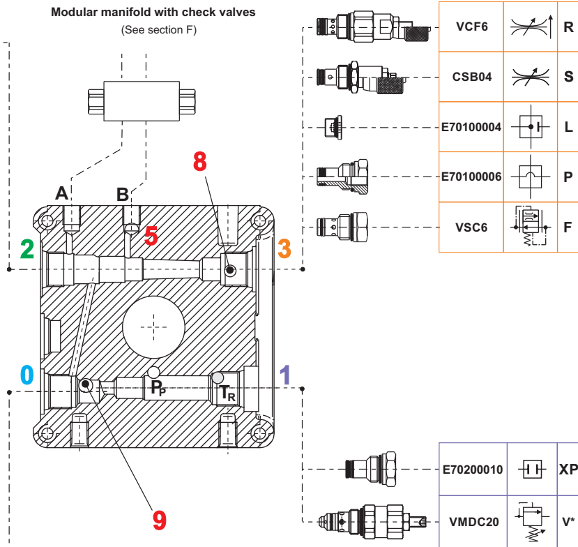
Hydraulic scheme
